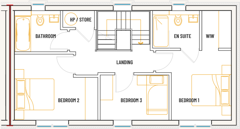
SECOND FLOOR
